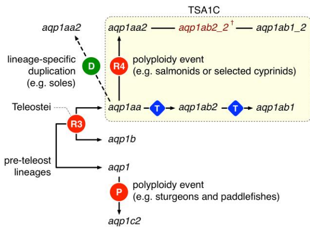
FIG. 2. The origins of multiple aquaporin-1 orthologs in fishes. Whole genome duplication (polyploidy) events (R3, R4, and P), respectively, generated aqp1b ohnologs in teleosts, a paralogous TSA1C in paleotetraploid salmonids and allotetraploid cyprinids and aqp1c2 in chondrosteian sturgeons and paddlefishes. Tandem duplication (T) gave rise to the teleost aqp1ab2 and aqp1ab1 paralogs. Conversely, lineage-specific duplication (D) generated the aqp1aa2 paralogs in soleid and cynoglossid flatfishes.
