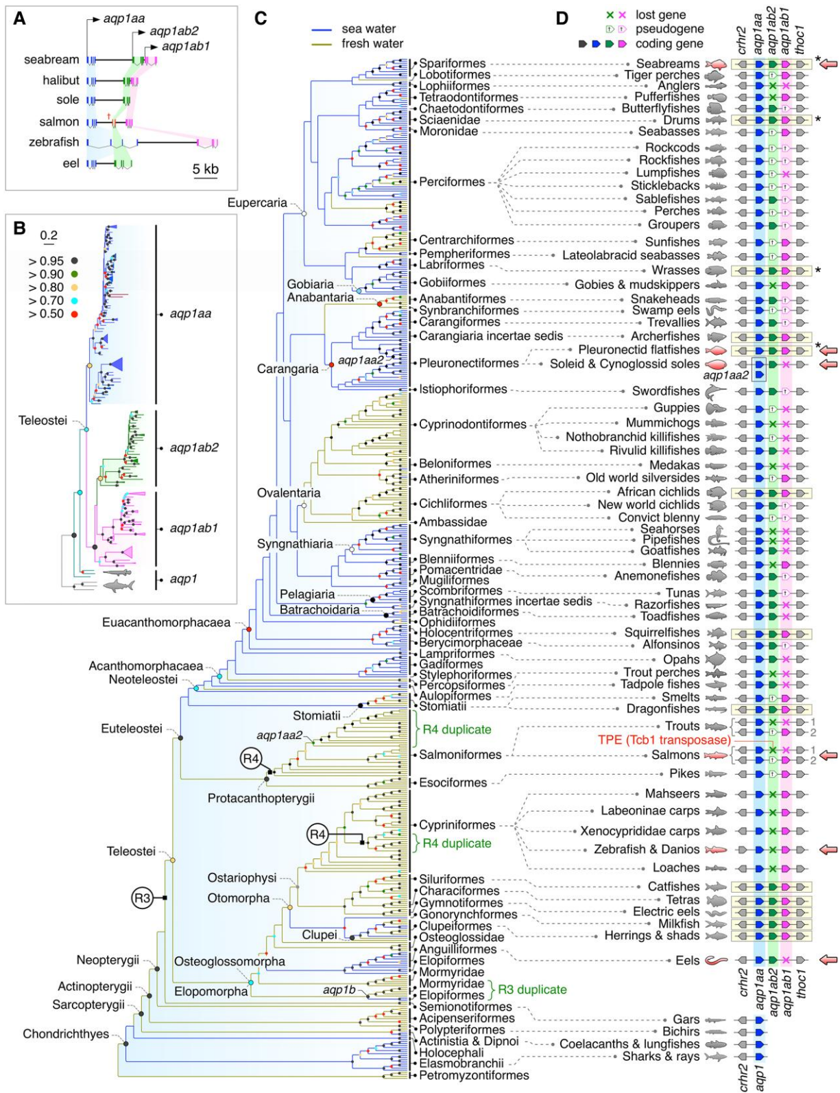
Fig. 1. The origin of the TSA1C. (A) Genomic organization of the TSA1C in distantly related teleosts drawn to scale. Canonical aqpa1aa , -1ab2 , and -1ab1 genes consist of four exons (blue, green, and magenta bars, respectively), while pseudogenes vary from premature stop codons to highly degraded fragments (e.g., salmon † ). In cypriniform teleosts (e.g., zebrafish) aqpa1ab2 is absent, while in anguilliform teleosts (e.g., eel) aqpa1ab1 is absent. (B) Bayesian majority rule consensus tree of the TSA1C coding sequences rooted with chondrichthyan aqp1 . The tree is inferred from 20 million Markov Chain Monte–Carlo (MCMC) generations (nucmodel = 4by4, nst = 2, rates = gamma) of 239,282 aligned nucleotide sites aligned by codon. Support values shown at each node (colored dots) are Bayesian posterior probability ranges shown in the key. The scale bar indicates the expected rate of substitutions per site. (C) Bayesian majority rule consensus tree of piscine aqp1 orthologs rooted with hyperoartian aqp01 . The tree is initially inferred from 100 million MCMC generations (nucmodel = 4by4, nst = 2, rates = gamma) of 399,429 aligned
