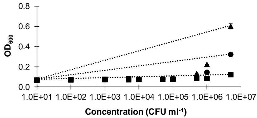
Fig. 2 Initial turbidity values obtained during the optimisation of the inoculum size used in the Bioscreen assays. Three formulations are represented: Candifruit (■); potato starch formulation (▲); and maltodextrin formulation (●). Linear regression for each formulation are represented with the dotted lines. Liquid SGJ media with continuous shaking treatment was used. Values are means of 5 readings recorded every 2 min during the first 10 min after inoculation. Three wells were used for each formulation. Error bars indicate standard errors of the means. Where bars are not shown, they were smaller than symbol size.
